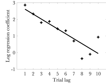
Figure 4: Log-transformed lag regression coefficients. Based on regression coefficients taken from Bayer and Glimcher (2005).
