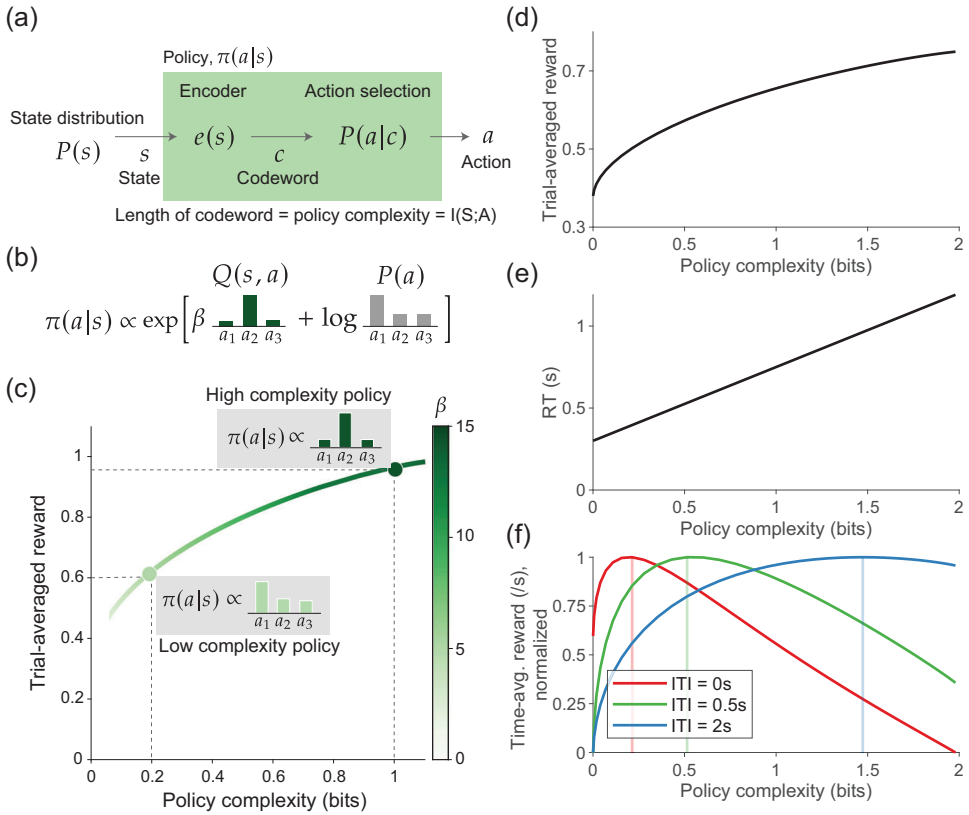
Fig. 1. The policy compression framework. (a) The policy as a communication channel. A state distribution P(s) generates states s that are encoded into memory, yielding a codeword c . The codeword is then mapped onto an action a according to P(a|c) . Together, encoding and action selection produce the policy \pi(a|s) . (b) The optimal policy includes a state-dependent term, Q(s, a) , and a state-independent term, \log P(a) . The \log P(a) term biases choices toward actions frequently chosen across all states. The \beta parameter determines the relative contribution of Q(s, a) and \log P(a) , controlling the policy's state-dependence. (c) The \beta parameter increases monotonically with policy complexity. We highlight two optimal policies at different policy complexity levels. The optimal policies trace out the reward-complexity frontier, which delimits achievable performance for a given policy complexity. (d) Reward-complexity frontier for Experiment 1. (e) Proposed linear relationship between RT and policy complexity. (f) Time-averaged reward as a function of policy complexity for each ITI under the linear RT relationship in (E); the policy complexity that maximizes time-averaged reward for each condition is highlighted (vertical lines). Panels (A–C) adapted from Lai and Gershman (2024); Panels (D–F) adapted from Liu, Lai, Gershman, and Bari (2025).
