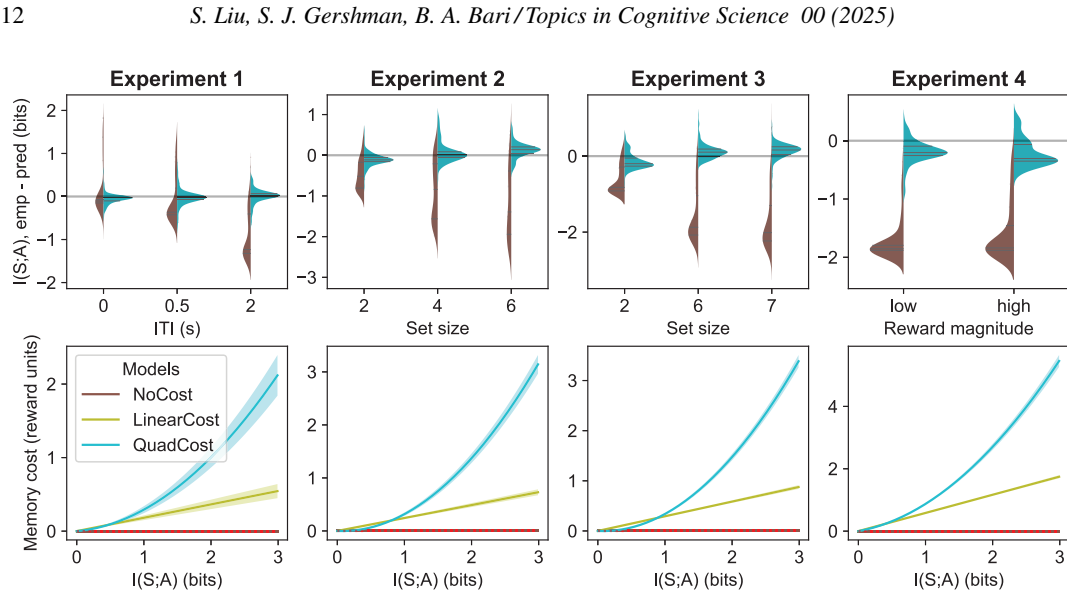
Fig. 4. Mental cost modeling results. Columns 1–4 correspond to Experiments 1–4. Colors denote models. Row 1: Violin plots of the difference between predicted and empirical I(S; A) . Densities to the left and right of the vertical line correspond to the NoCost and QuadCost models. Row 2: Mean \pm SEM of fitted MentalCost ( I(S; A) ) functions across participants.
