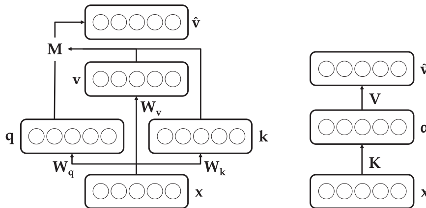
Figure 1. Two architectures for key-value memory
