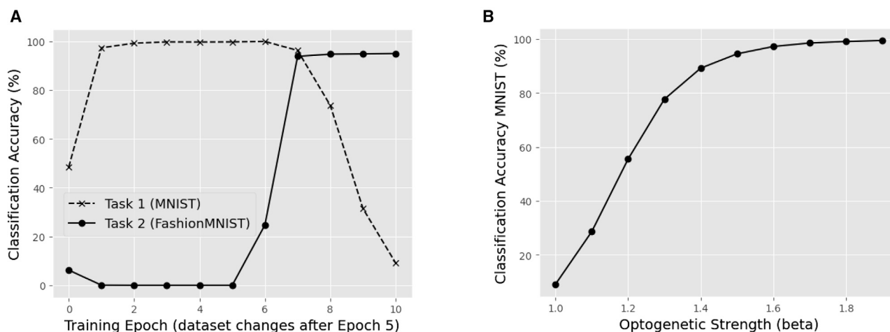
Figure 3. Forgetting and reactivation of memory events
